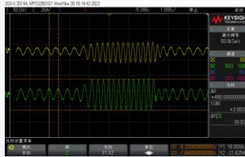
Current/voltage waveform in low speed full-load operation
