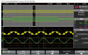
Current/voltage waveform under abrupt load
