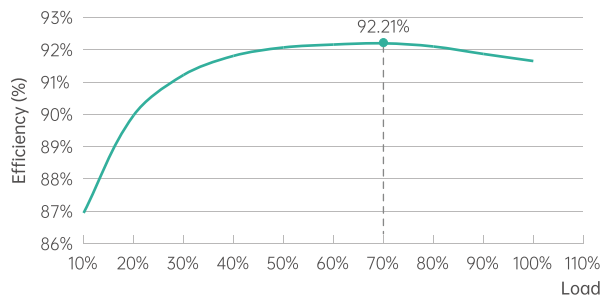
Rectifier efficiency curve
