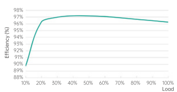
Efficiency curve
