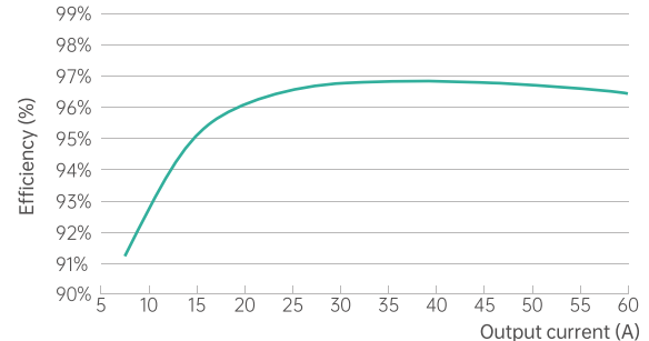
Efficiency curve
