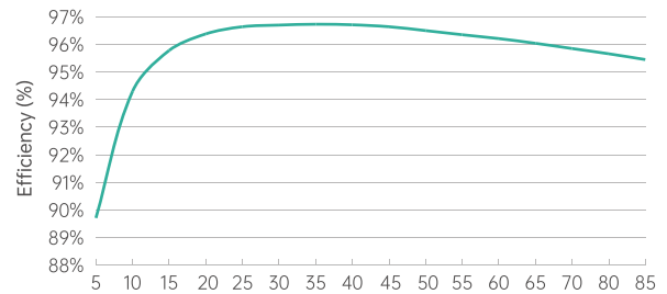
Efficiency curve
