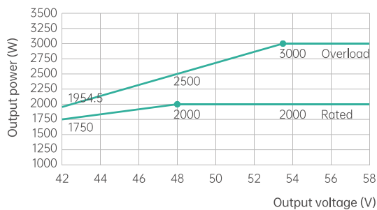
Output overload capacity
