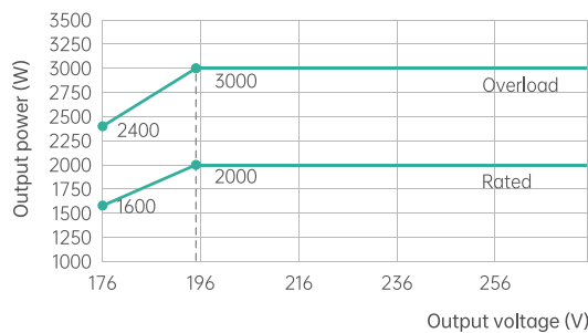
Output overload capacity
